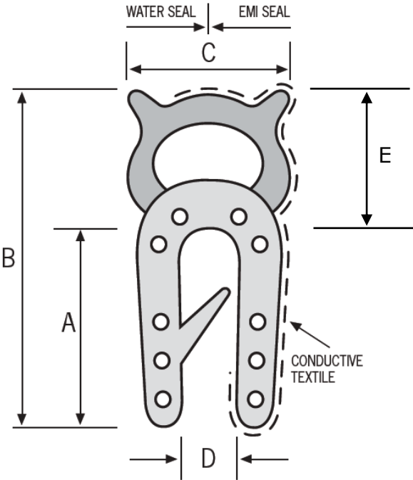
Dimensions for Profile Type: 6590
